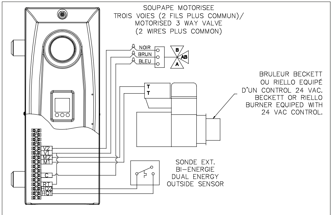
Figure 10: Installation bi-énergie
